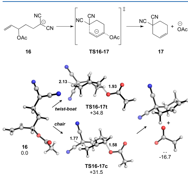
Figure 6. Stationary points calculated for the ICD reaction lacking a Michael acceptor.
