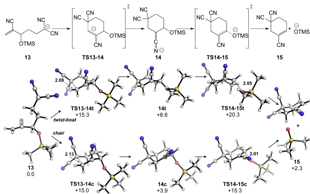
Figure 3. Stationary points calculated for the ICD reaction of OTMS derivative 13.
