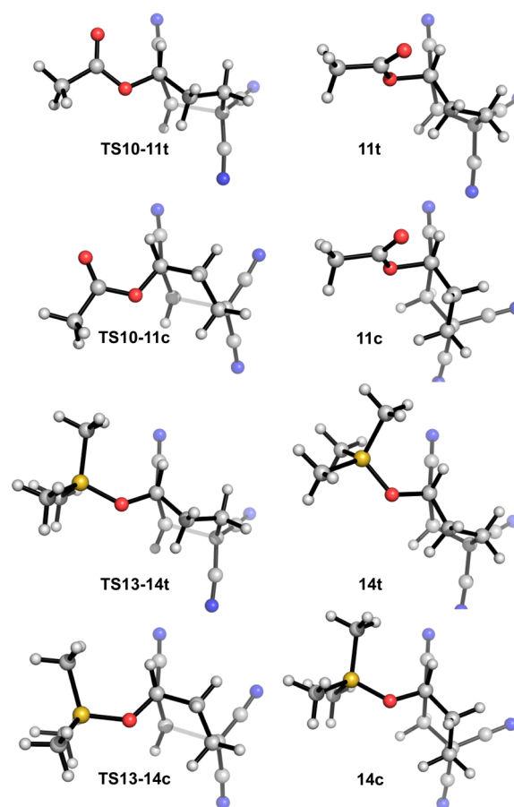
Figure 5. Addition transition states TS10–11 and TS13–14 and intermediates 11 and 14 in the twist-boat and chair conformations, showing the dihedral angle between the cyano group and leaving group.
