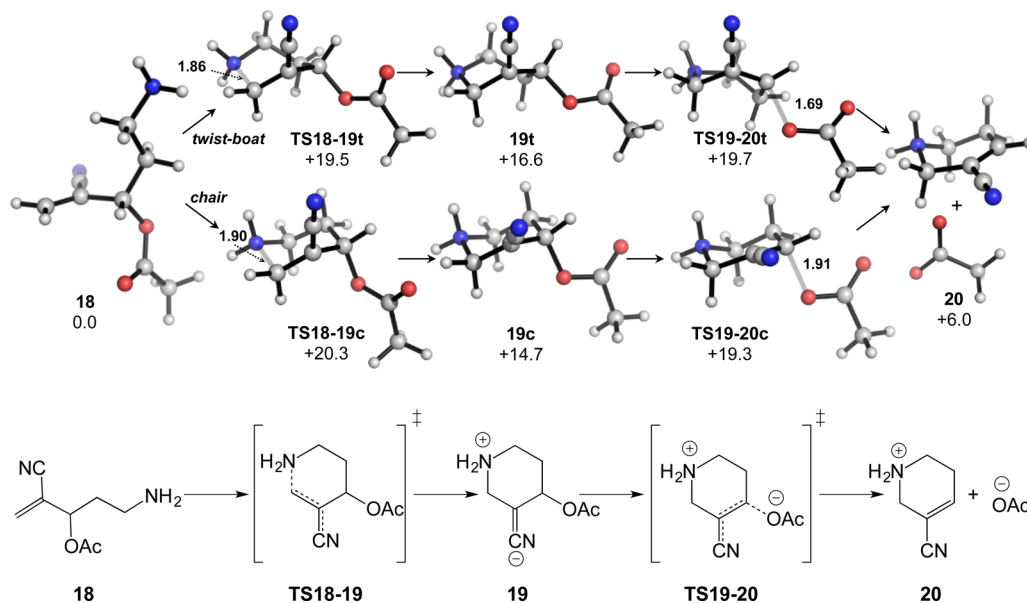
Figure 7. ICD reaction mechanism with an amine nucleophile.
