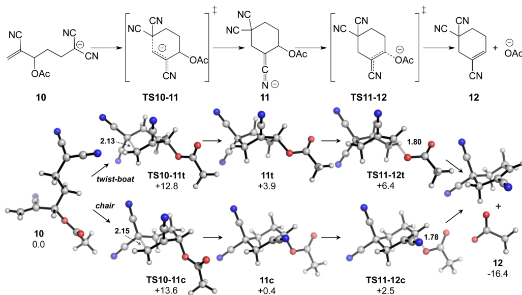
Figure 2. ICD reaction stationary points.
