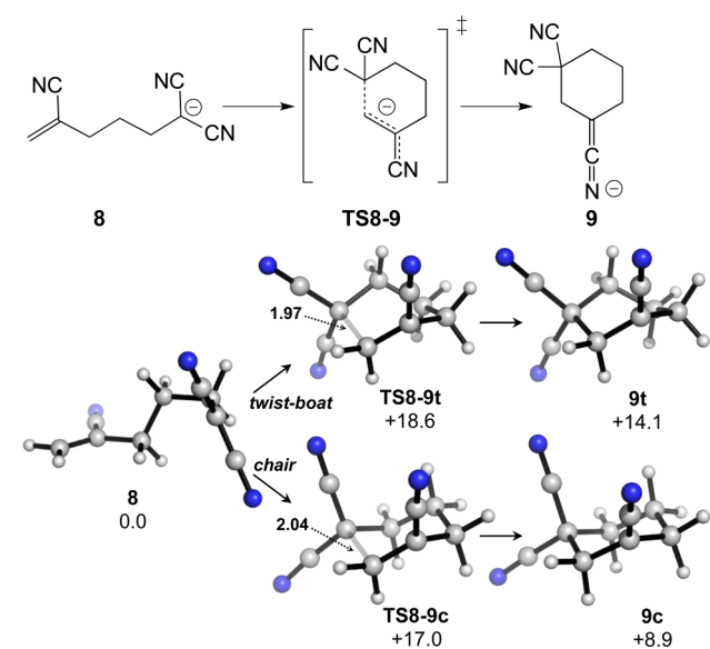
Figure 1. Reactant, transition states, and product for the ICD reaction of malononitrile anion with an acrylonitrile moiety.
